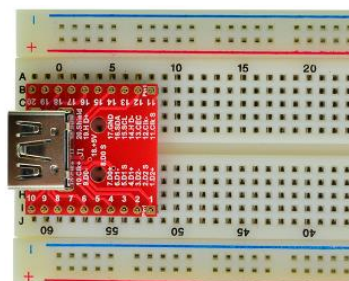
Figure 2: Example of connecting the HDMI-AF-BO-V1A stably on a breadboard
