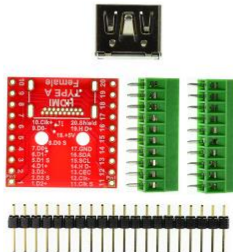
Figure 1: Parts inside the kit
